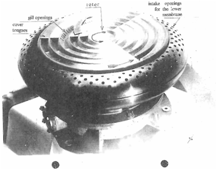
Fig. 31: Repulsine patent
